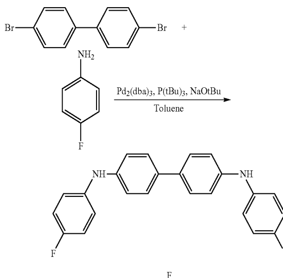
Reaction Scheme 5
