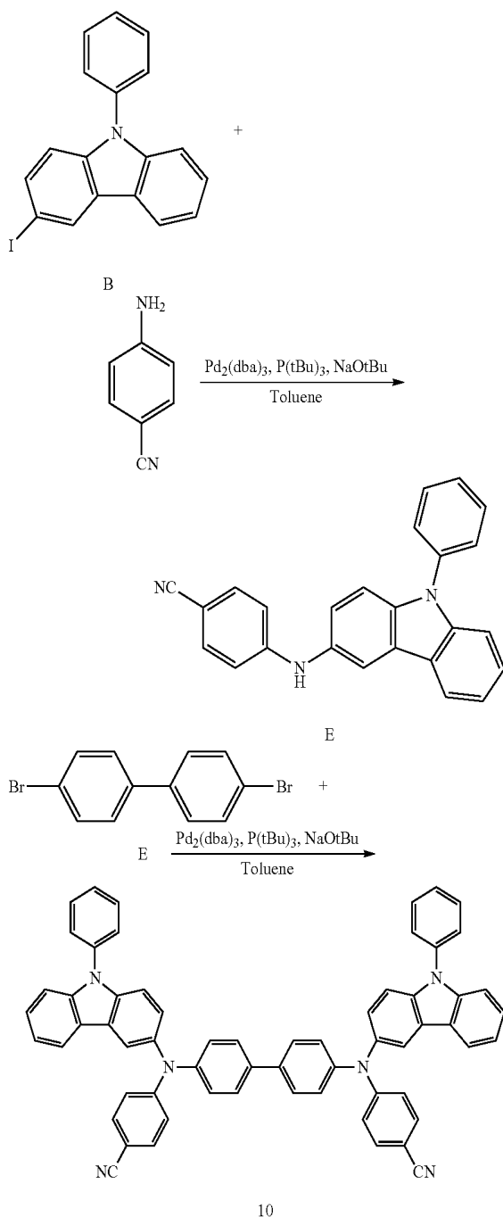
Reaction Scheme 4
