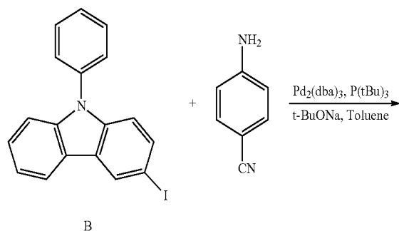
Reaction Scheme 8
