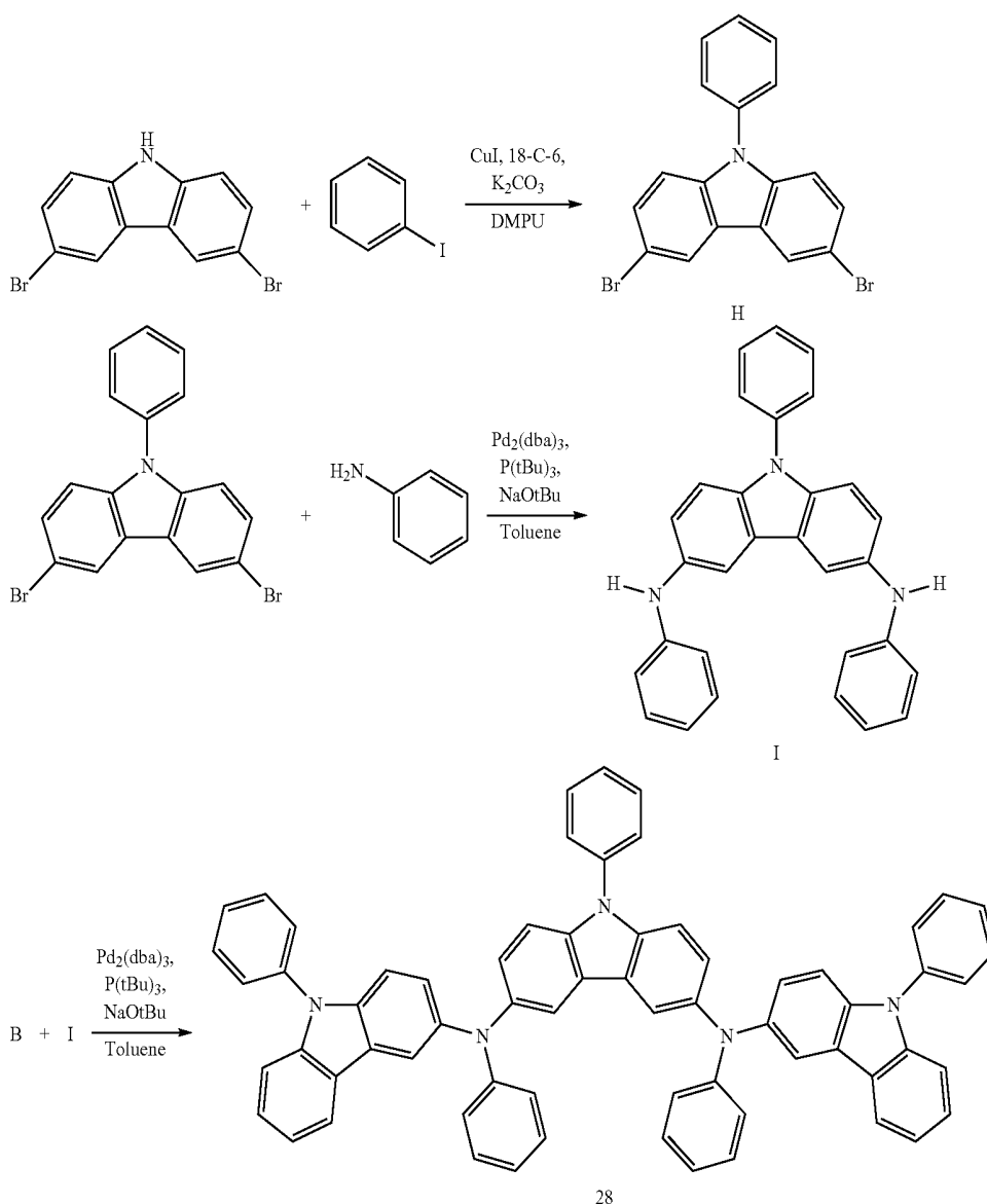
Reaction Scheme 7
